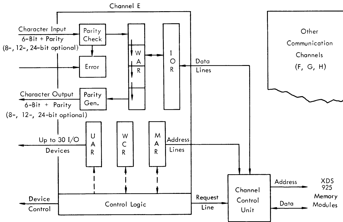
Figure 4-2. XDS 925 Direct Access Communication Channel, Block Diagram
