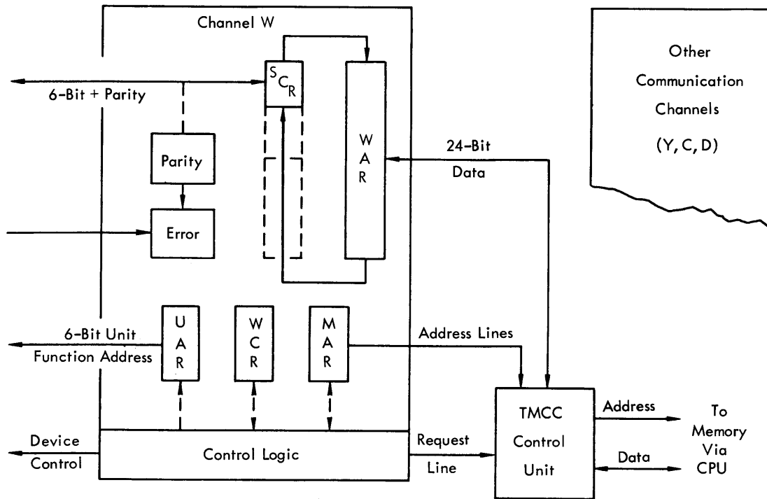
Figure 4-1. XDS 925 Time-Multiplexed Communication Channel, Block Diagram
